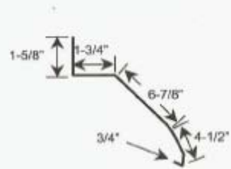
17. Cannonball Double Track Cover
