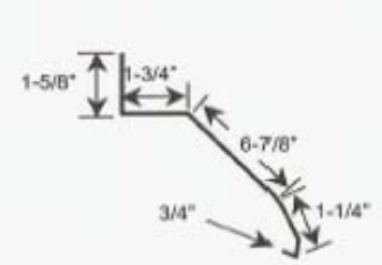
17. Cannonball Track Cover
