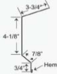
13. Fascia Eave Trim
